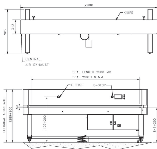
Dimension sketch of PSR (PLUS) XL 2500 without vacuum system
